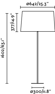
Textile diffuser
