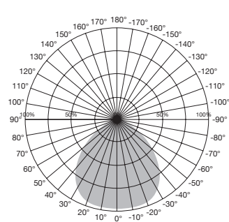
Beam Angle: 120°
