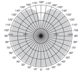
Beam Angle: 300°
