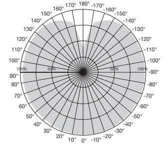
Beam Angle: 320°
