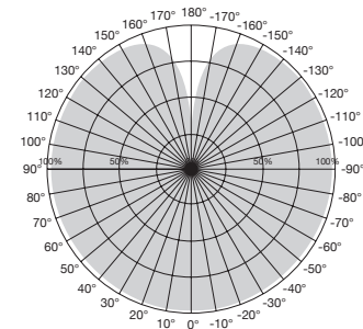
300° Illumination
