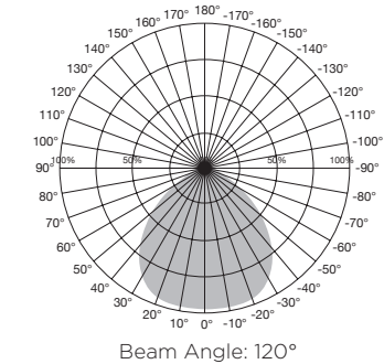
Beam Angle: 120°
