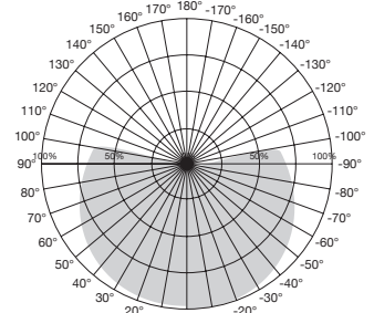
Beam Angle: 100°
