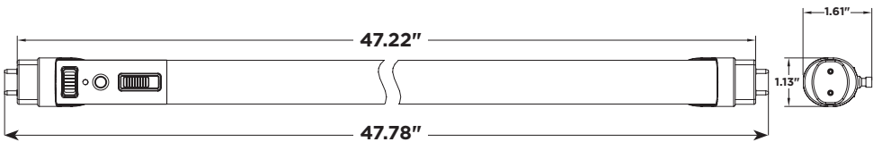
DIMENSIONAL DIAGRAM
