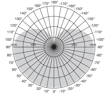
Beam Angle: 230°
