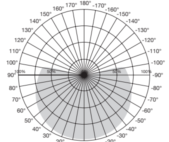
Beam Angle: 103°
