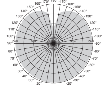
Beam Angle: 320°
