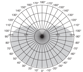
Beam Angle: 220°
