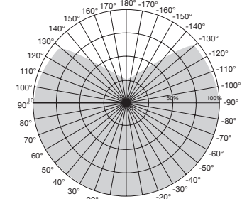
Beam Angle: 135°
