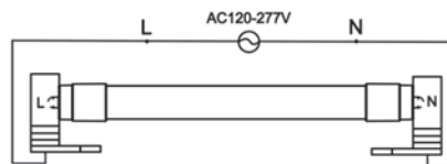
Wiring Diagram
