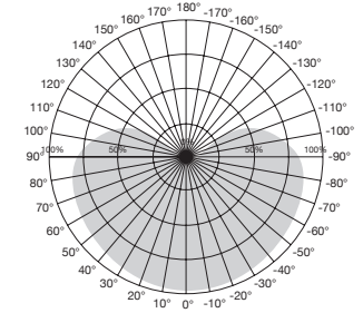
Beam Angle: 175°
