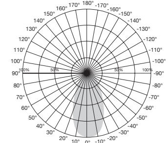
Beam Angle : 40°
