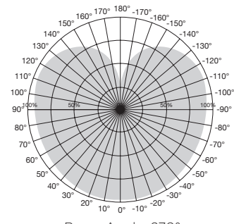
Beam Angle: 270°
