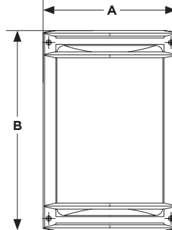
LED Outdoor Rectangular Bulkhead Fixture
