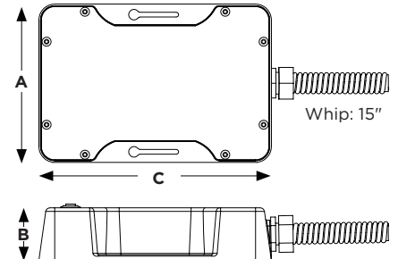
65-638, 65-639 8W/15W Emergency Backup
