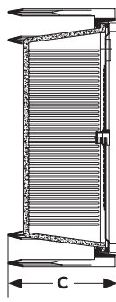
LED Outdoor Rectangular Bulkhead Fixture
