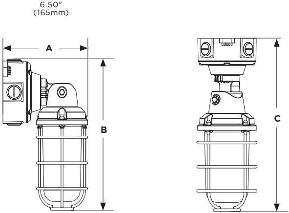
Fixture adjusts a full 90° in multiple increments.
