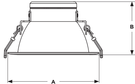
10 inch LED Commercial Downlight
