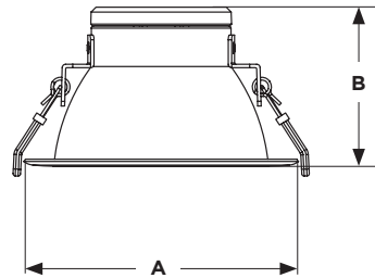
6 inch LED Commercial Downlight
