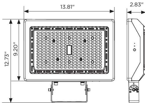
150W With trunnion mount
