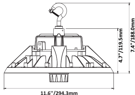
100W/120W/150W 277-480V
