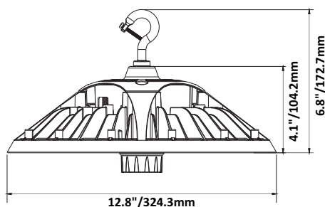
200W/240W 120-277/347
