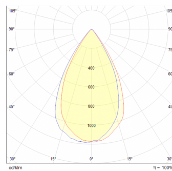
Focus 45W 36°
