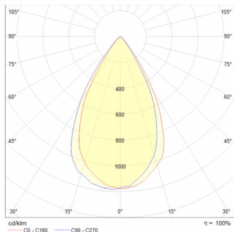
Focus 30W 60°
