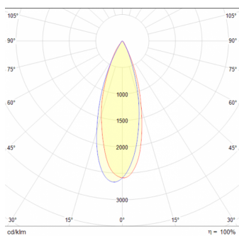
Focus 30W 36°
