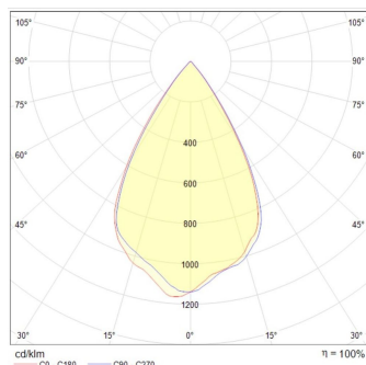
Focus 15W 60°
