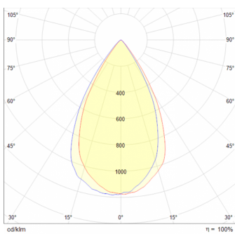
Focus 45W 60°
