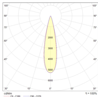
Focus 15W 24°
