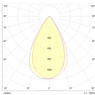
Focus 45W 24°
