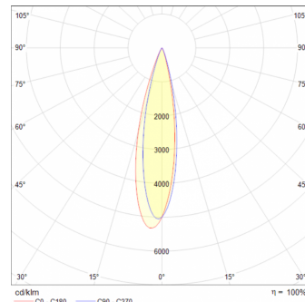
Focus 30W 24°
