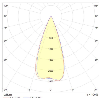
Focus 15W 36°
