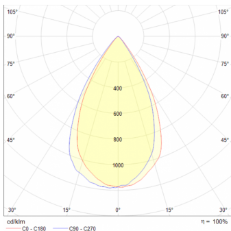
Focus 45W 60°
