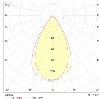
Focus 45W 36°
