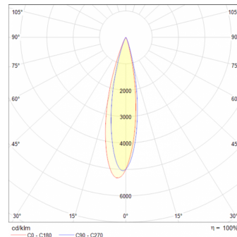
Focus 30W 24°
