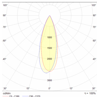
Focus 30W 36°
