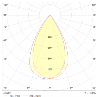
Focus 45W 24°
