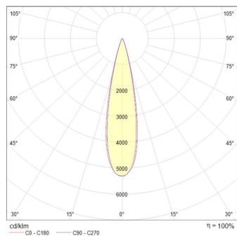
Focus 15W 24°
