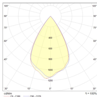
Focus 15W 60°
