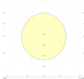
Magnettrack Pro Lineal 35W 110°
