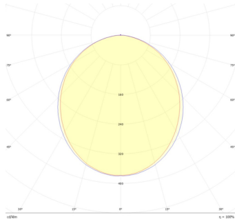
Magnettrack Pro Lineal 15W 110°
